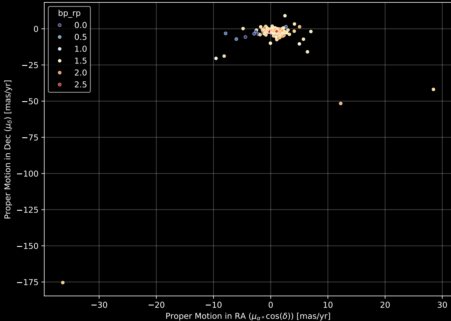
APOGEE DR17 Field: [161+04] Proper Motion Diagram (n= 193)
