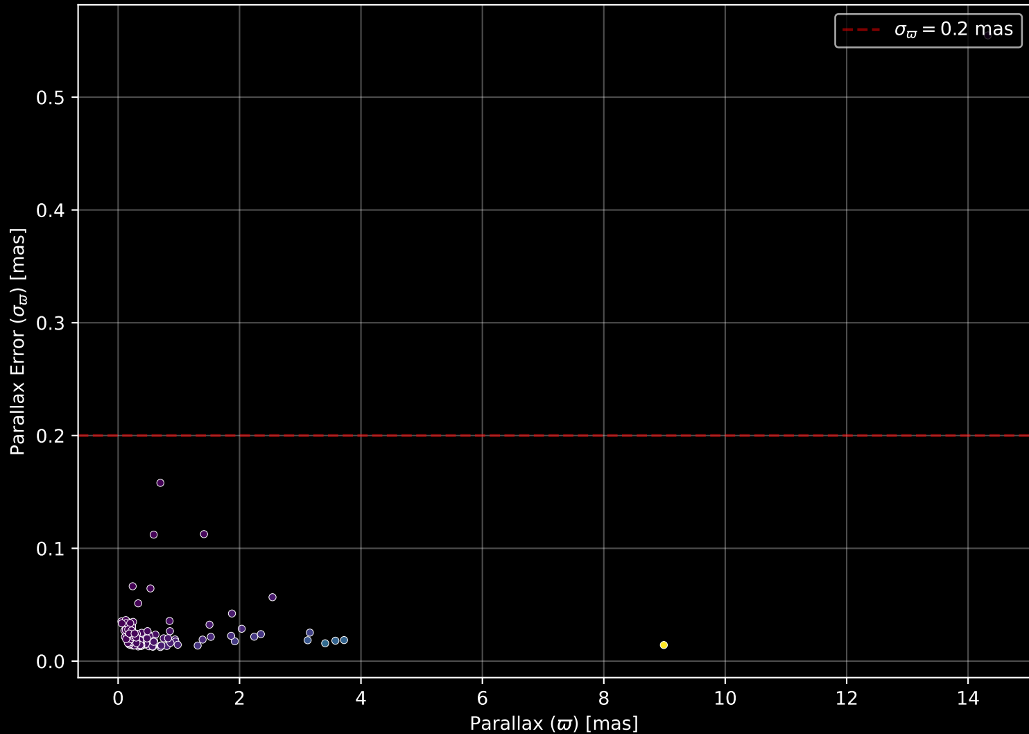
APOGEE DR17 Field: [161+04] Parallax Quality (n= 193)
