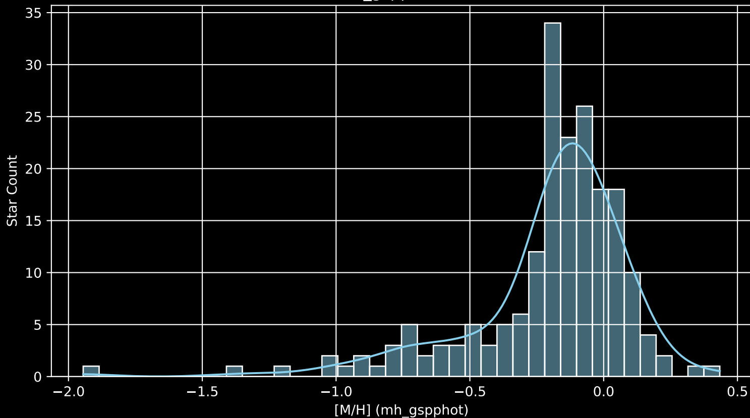
APOGEE DR17 Field: [161+04 [M/H] (mh_gspphot) (n= 193)
