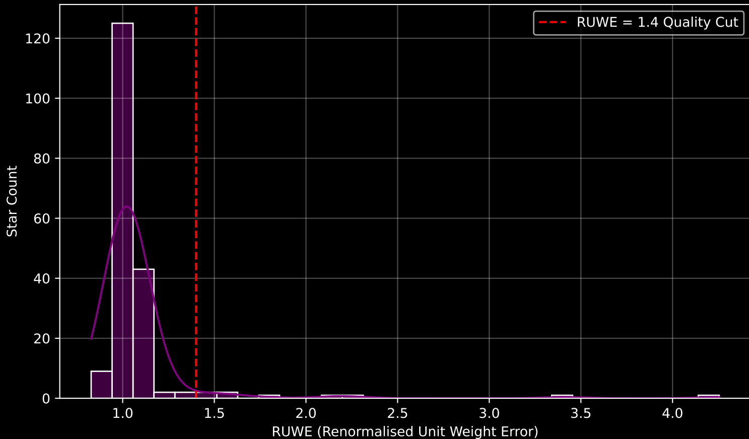
GAPOGEE DR17 Field [161+04] RUWE Distribution (n= 190)
