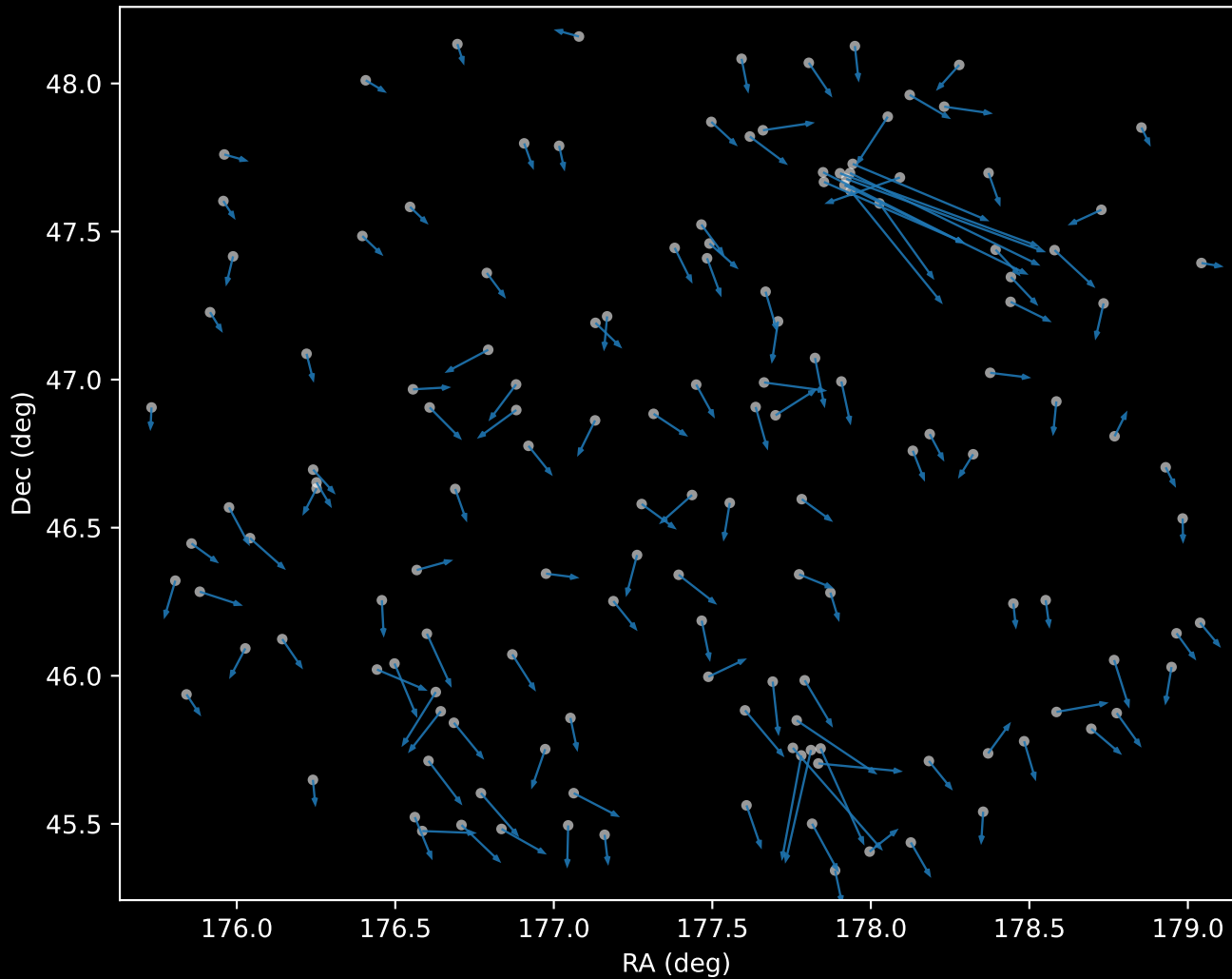
APOGEE DR17 Cluster 0 Proper Motion Vectors (n=145)
