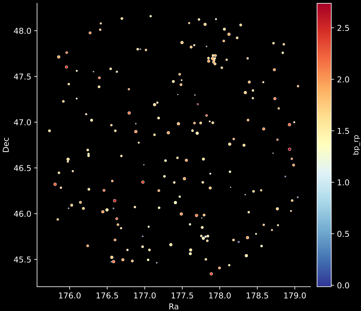
APOGEE DR17 Field: [161+04] Stars: 193
